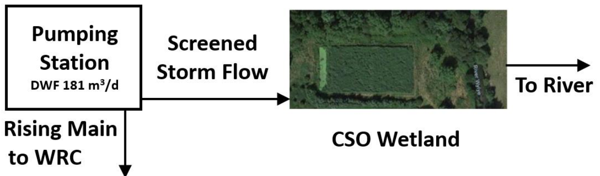
Figure B6. Schematic process flow at Hanging Langford Pumping Station
